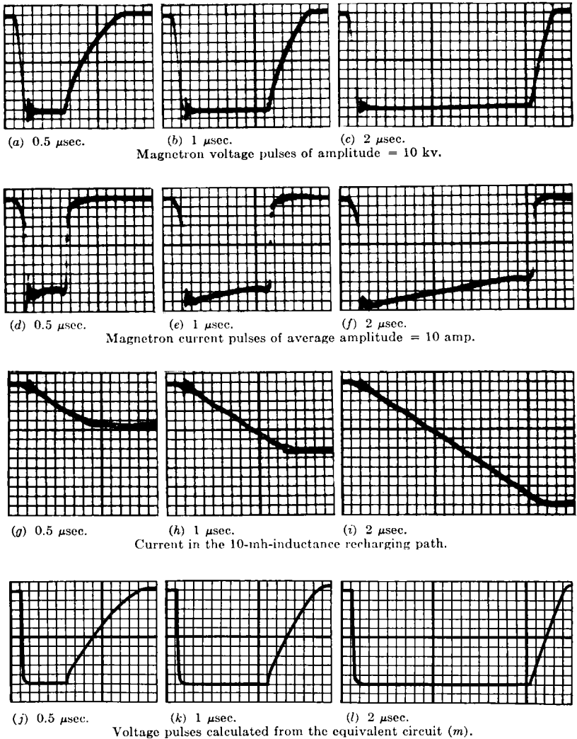
FIG. 2-25.—Oscilloscope traces and calculated pulse shapes for a hard-tube pulser with a magnetron load, a 10-mh inductance as the recharging path, a shunt diode, and C_s = 115 \mu\text{mf} . Voltage pulses were calculated from the equivalent circuit (m) and S_T closed 0 < t < \tau , S_I closed for V_{ba} > 0.7E_{tb} , S_M closed when S_I opens and until V_{ba} = 0 , S_d closed for negative values of V_{ba} . Sweep speed: 10 div. = 1 \mu sec.
